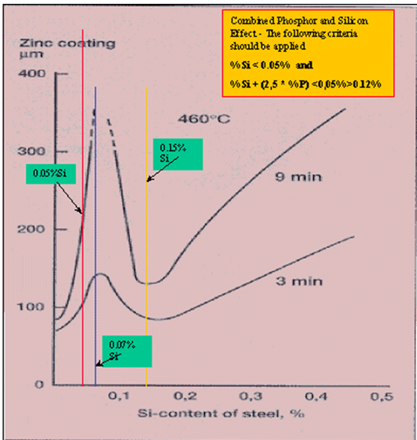
Figure 22. Relationship between silicon content of steel and thickness of zinc coating for dipping times of 9 and 3 minutes respectively at 460°C. The curves are average curves. Significant variations can occur between steels with the same Si content, but from different charges. The high reactivity is between 0.05 and 0.12% Si. This called the Sandelin Effect.
